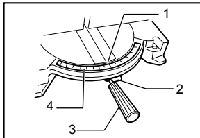
1. Pointer 2. Lock lever 3. Grip 4. Miter scale
